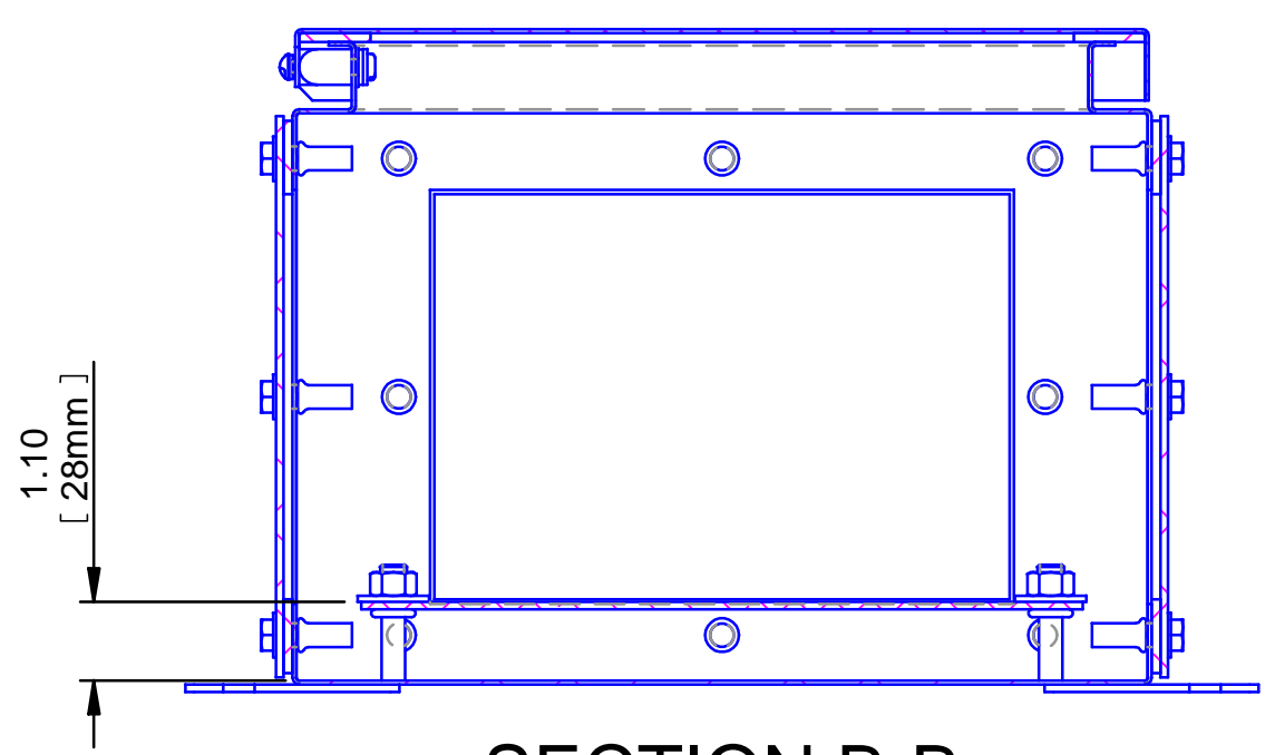
SECTION B-B
