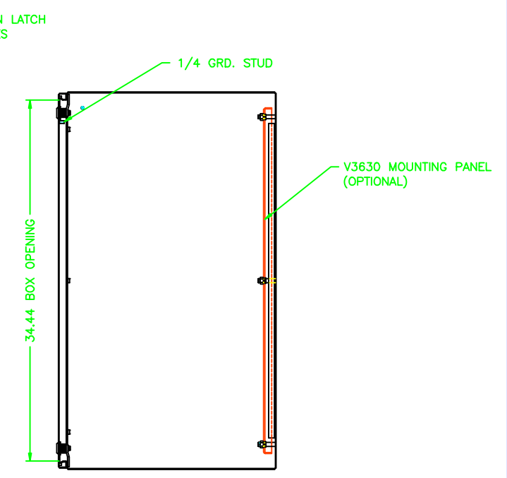
SECTION C-C
